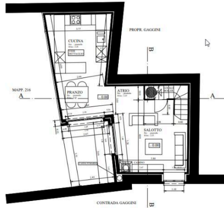
PIANO TERRENO
